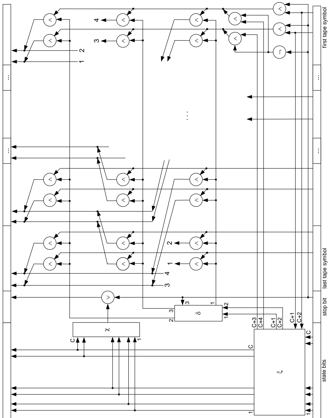
Fig. 1. Single step of turing machine as a shrink function
